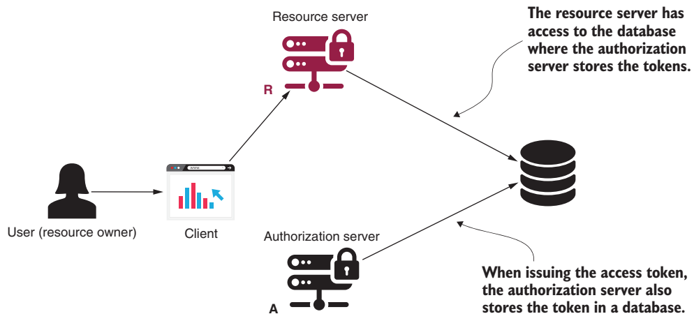
Figure 14.3 Blackboarding. Both the authorization server and the resource server access a shared database. The authorization server stores the tokens in this database after it issues them. The resource server can then access them to validate the tokens it receives.
