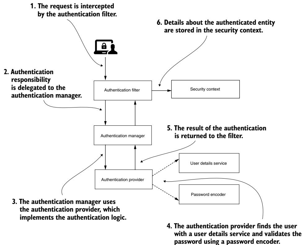
Figure 2.2 The main components acting in the authentication process for Spring Security and the relationships among these. This architecture represents the backbone of implementing authentication with Spring Security. We'll refer to it often throughout the book when discussing different implementations for authentication and authorization.
