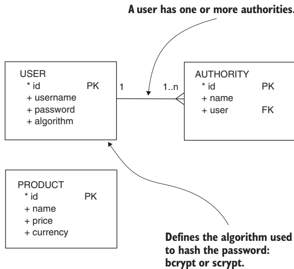
Figure 6.3 The entity relationship diagram (ERD) of the database for the current example. The user table stores the username, password, and the algorithm used to hash the password. Also, a user has one or more authorities that are stored in the authority table. A third table, named product, stores the details of the product records: a name, a price, and a currency. The main page displays the details of all the products stored in this table.
