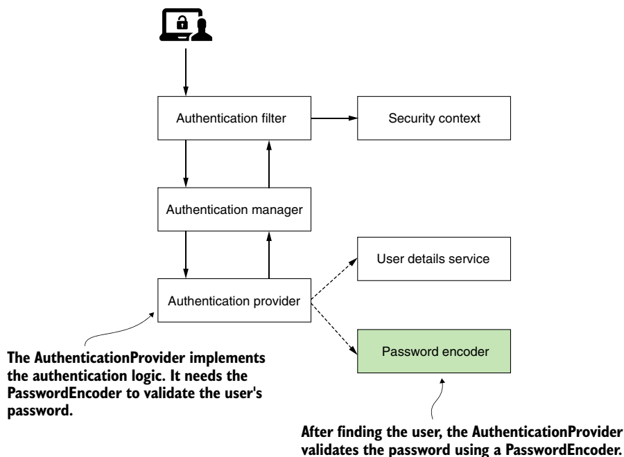
Figure 4.1 The Spring Security authentication process. The AuthenticationProvider uses the PasswordEncoder to validate the user's password in the authentication process.
