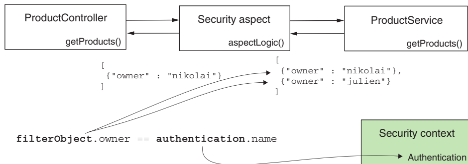
Figure 17.8 In the SpEL expression used for authorization, we use filterObject to refer to the objects in the returned collection, and we use authentication to refer to the Authentication instance from the security context.
