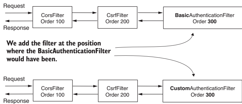
Figure 9.13 We add our custom authentication filter at the location where the class BasicAuthenticationFilter would have been if we were using HTTP Basic as an authentication method. This means our custom filter has the same ordering value.
